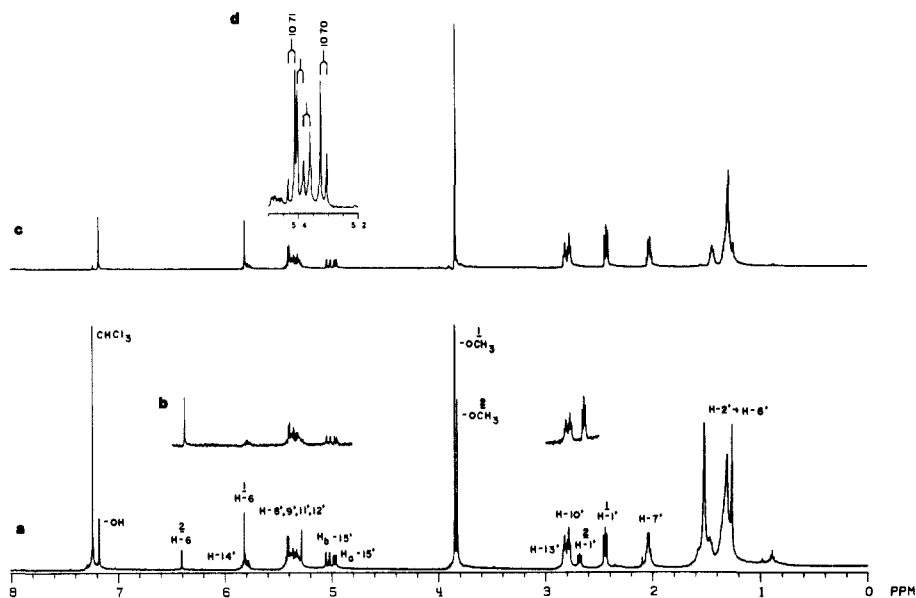
Figure 1. ^1\text{H-NMR} (500 MHz) spectra in 500 \mu\text{L} of \text{CDCl}_3 of (a) Sorghum crude exudate (1 mg), (b) hydroquinone 2 obtained by reducing 1 (1 mg) with zinc dust/HOAc, and (c) quinone 1 (4 mg), (d) triple-frequency irradiation of H-7', -10', and -13' simplified the vinylic region to two AB patterns with J = 10.7 Hz.
